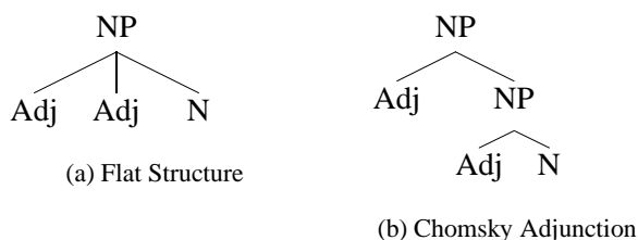
Figure 10: Two Representations for Optional, Repeatable Constituents
